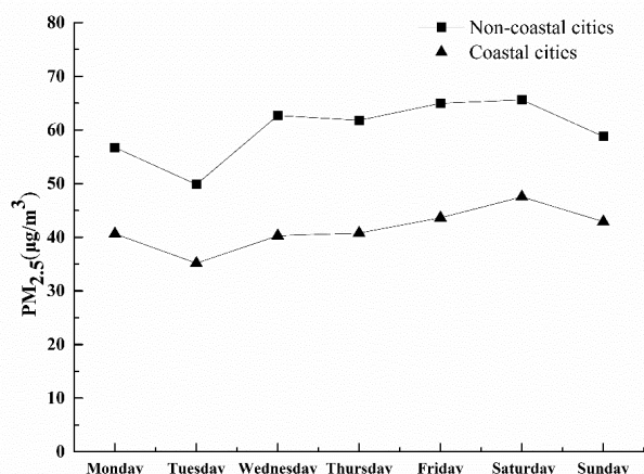
Fig. 5. PM 2.5 weekly changes in coastal and non-coastal cities.
