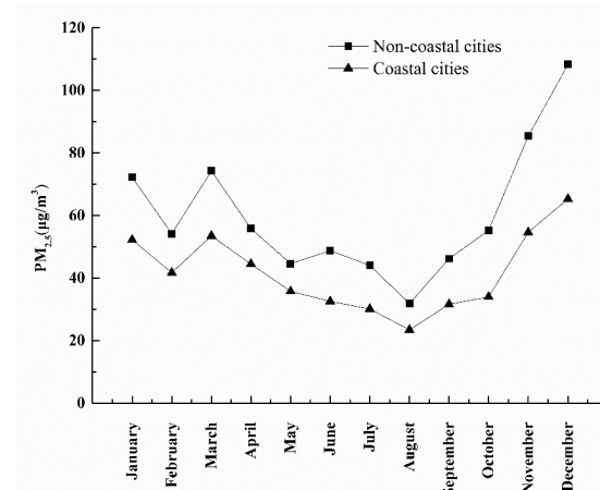
Fig. 4. Coastal and non-coastal city PM_{2.5} monthly changes.
